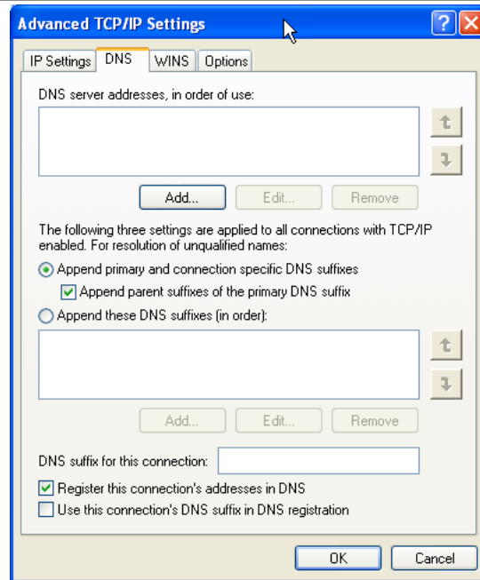
Figure 8.4. DNS Configuration.
