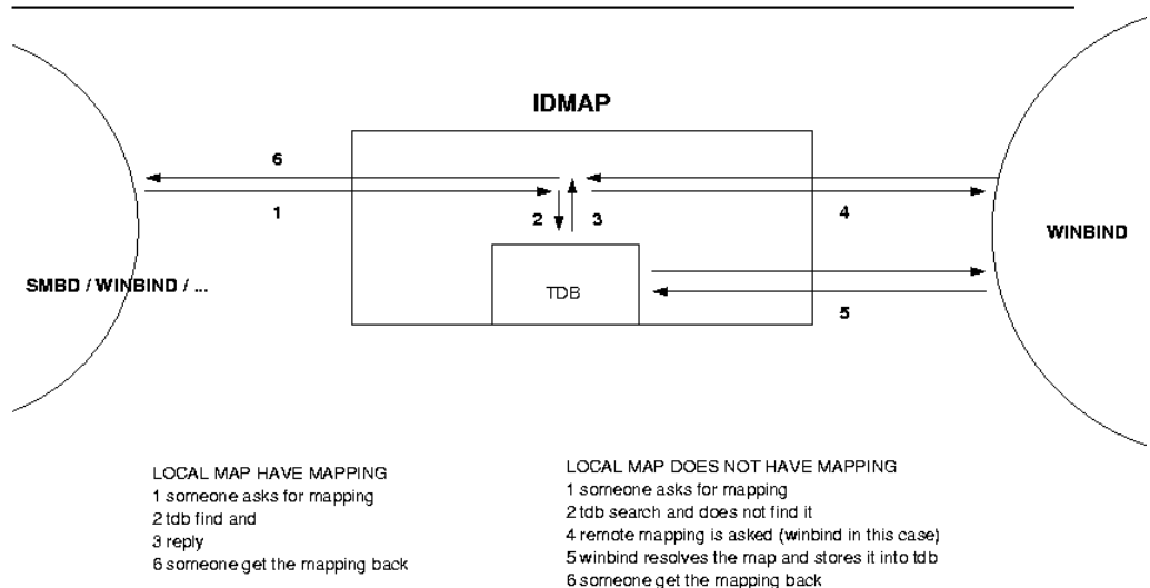
Figure 24.1. Winbind Idmap
