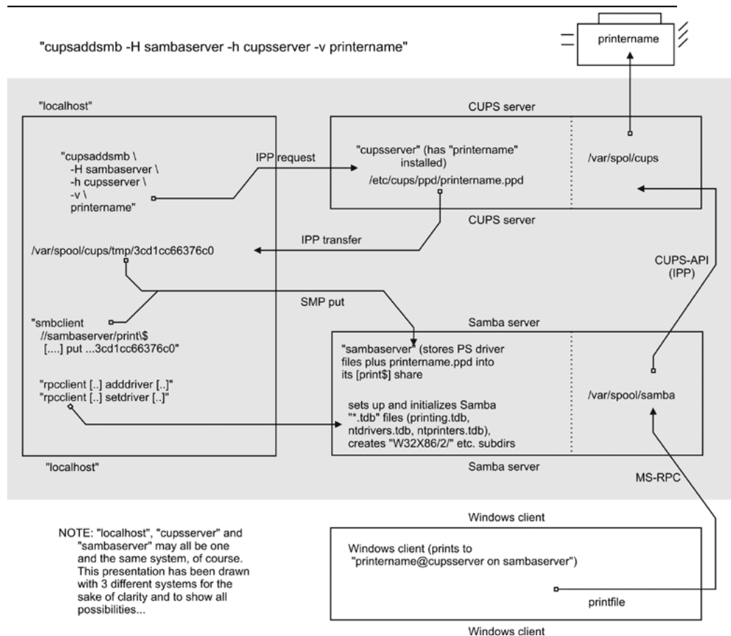
Figure 22.16. cupsaddsmb Flowchart.
